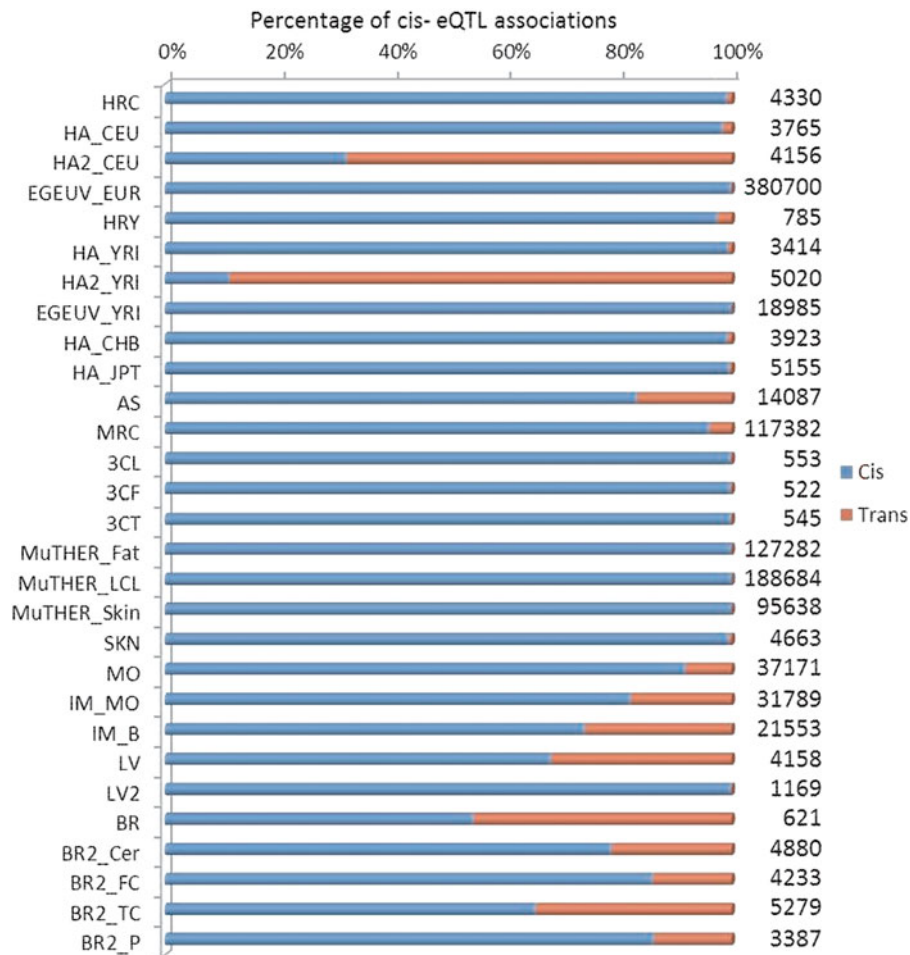
SUPPLEMENTARY FIG. S1. Fraction of cis- and trans-eQTL associations in each dataset. The number at the end of each row is the total number of eQTL associations. The fraction of associations classified as trans-eQTL in the HA2 study is much higher than others as a result of that study considering all associations out to 4 Mb, as opposed to the more usual 1 Mb. eQTL, expression quantitative trait locus.
