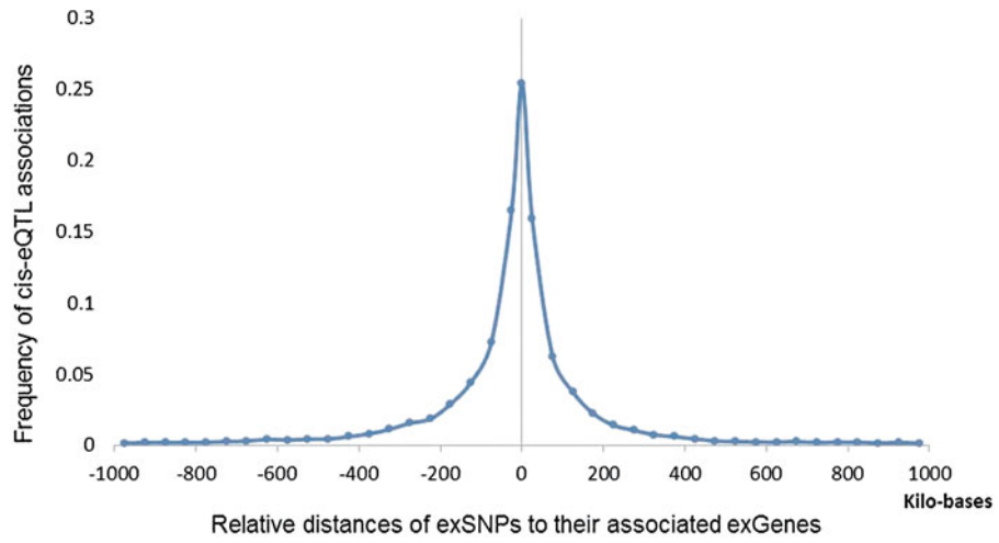
SUPPLEMENTARY FIG. S2. Distribution of distances between each cis-exSNP and the associated exGene. Most distances are relatively short—less than 200 kb.
