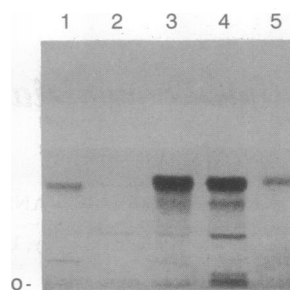
FIG. 1. Synthesis of Dol- ^{14}\text{C} ]Man by sec59 membranes. Washed membranes were prepared from sec59 cells that had been incubated 24^\circ\text{C} (lanes 1 and 3) or shifted to 38^\circ\text{C} (lanes 2 and 4) for 1 hr. Synthesis of Dol- ^{14}\text{C} ]Man was measured in the absence (lanes 1 and 2) or presence (lanes 3 and 4) of 20 \mu\text{g} of exogenous Dol- P . Radiolabeled lipids were extracted and separated by thin-layer chromatography on silica gel 60 with chloroform/methanol/water (65:25:4 by volume) as solvent (0, origin). Lane 5, Dol- ^{14}\text{C} ]Man standard made by incubation of membranes from wild-type yeast with GDP- ^{14}\text{C} ]mannose and mammalian Dol- P .
