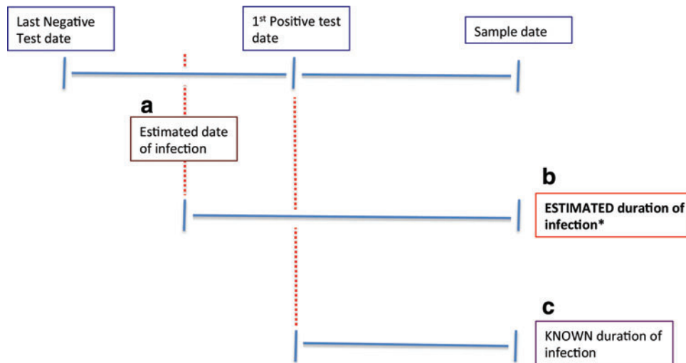
SUPPLEMENTARY FIG. S2. Definitions of computed variables. (a) Estimated date of infection: the midpoint between the last negative and first positive test in the surveillance. (b) Estimated duration of infection: time between the estimated date of infection and the sample date (months). This is the primary variable for the categorization of infections. (c) Known duration of infection: time between the first positive date and sample date (months). This is a secondary variable for the categorization of infections.
