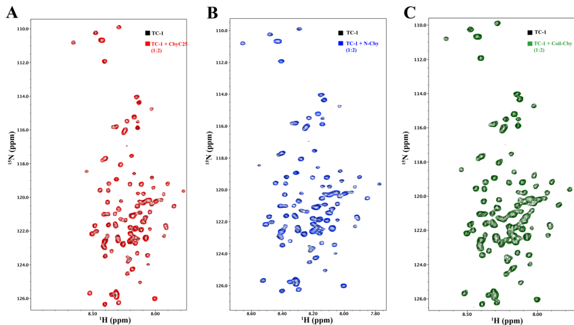
Supporting Information Figure 2. A. Overlay of the ^1\text{H} - ^{15}\text{N} HSQC spectra of TC-1 in the absence (black) and presence (red) of N-Cby at a 1:2 ratio (TC-1:N-Cby). B. Overlay of the ^1\text{H} - ^{15}\text{N} HSQC spectra of TC-1 in the absence (black) and presence (red) of CbyC25 at a 1:2 ratio (TC-1:CbyC25). C. Overlay of the ^1\text{H} - ^{15}\text{N} HSQC spectra of TC-1 in the absence (black) and presence (red) of Coil-Cby at a 1:2 ratio (TC-1:Coil-Cby).
