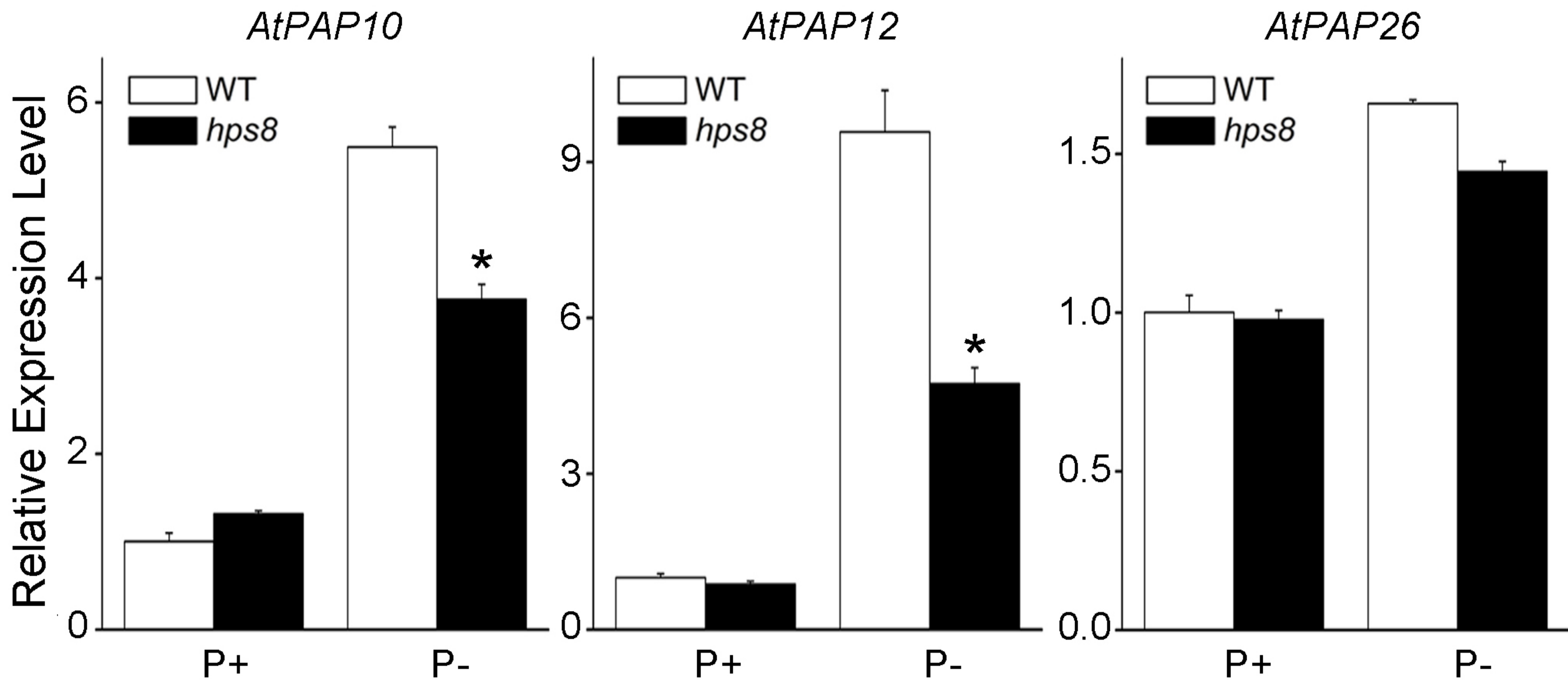
Figure S1. qPCR analysis of relative expression of AtPAP10 , AtPAP12 and AtPAP26 APase genes in roots of the WT and hps8 seedlings. Values represent means with SE of three replicates. Asterisks indicate significant difference ( p < 0.05 ) from the WT according to Student's t -test.
