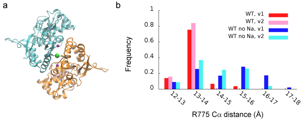
Supplementary Figure 4 Sodium unbinding initiates rearrangements of the LBD dimer interface that are associated with desensitization. (a) Top view of the crystal structure of the wildtype GluK2 LBD dimer showing two sodium ions (purple), one chloride ion (green), and the alpha carbons of both R775 residues (grey) adjacent to the dimer interface. The distance of the line connecting these carbons reflects the separation of the upper lobes of subunits. (b) Inter-subunit R775 alpha carbon distance during 100 ns MD simulations in which the two bound sodium ions are either left in place or removed prior to the simulation.
