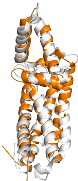
Helical-II
