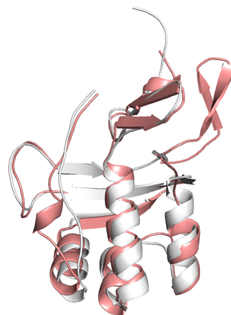
Nuc
