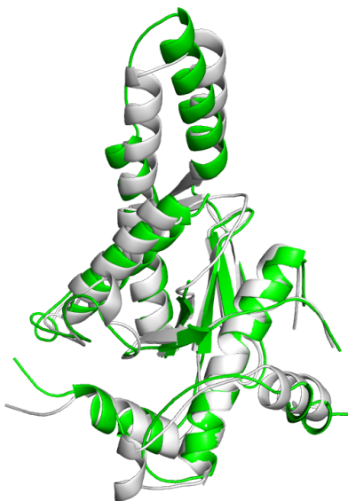
RuvC
