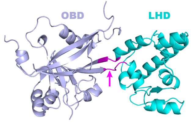
Cpf1-crRNA-DNA ternary complex
