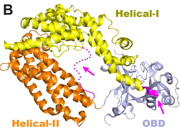
Cpf1-crRNA binary complex
