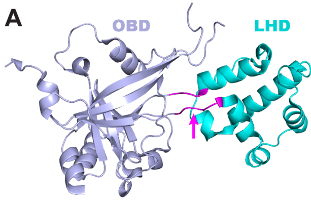
Cpf1-crRNA binary complex
