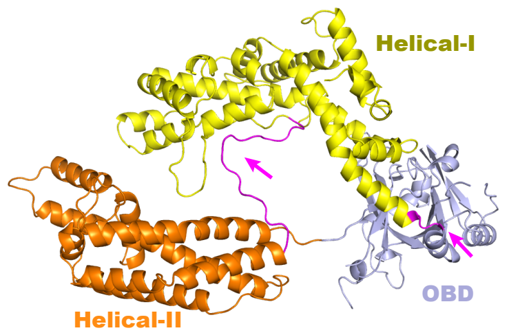
Cpf1-crRNA-DNA ternary complex
