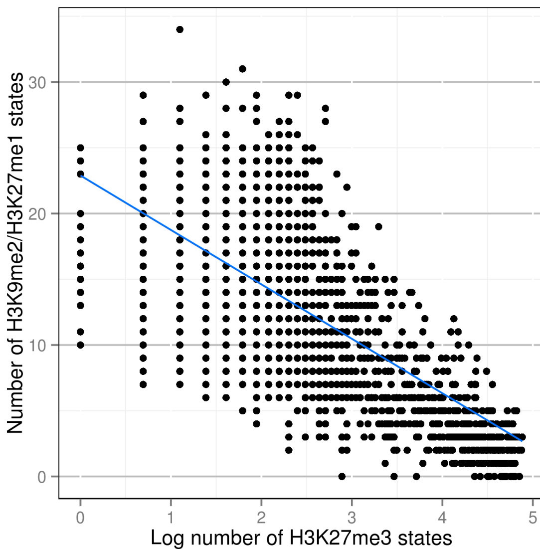
Figure S5: Relationship between distribution of H3K27me3 and H3K27me1/H3K9me2: Each spot represents a 0.5 Mbp bin containing the corresponding number of chromatin states for [H3k9me2+H3K27me1] and [H3K27me3] over the entire Barley genome. Log = natural logarithm.
