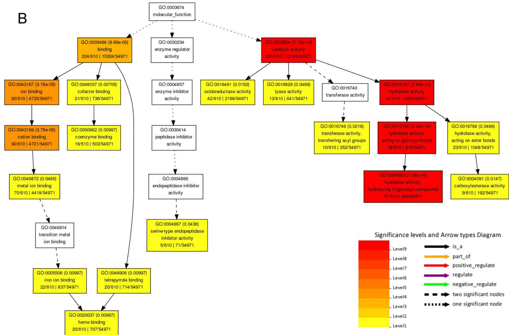
Fig. S4. GO analysis of the 622 DEGs in the three CMS lines. (A) GO enrichment of biological process; (B) GO enrichment of Molecular function.
