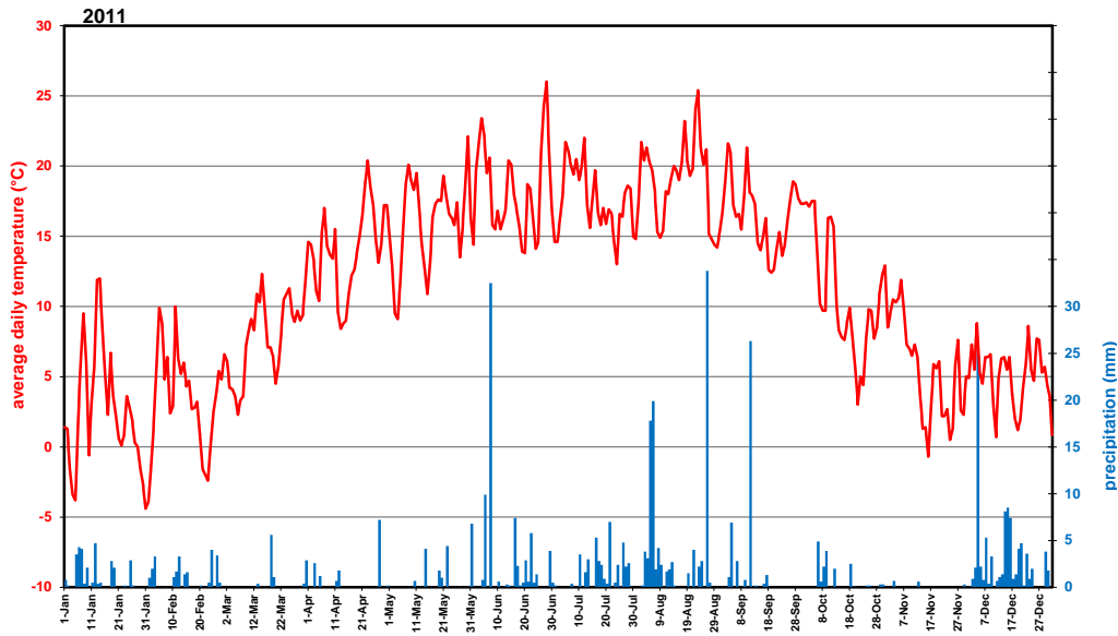
S2 Fig. Climatic conditions 2010 and 2011, obtained from a weather station of the German meteorological service DWD (Deutscher Wetterdienst) located next to the experimental vineyard in Geisenheim. The three sampling dates are marked with an arrow.
