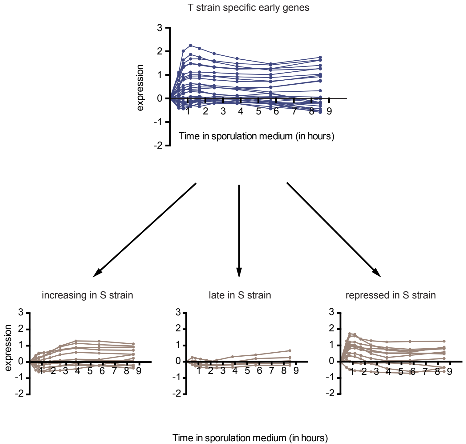
Figure S5. Genes showing early expression in T strain, show expression in later time points or are repressed in S strain. Gene expression is shown on Y-axis and time in sporulation medium is shown in X-axis. For gene list in each cluster see Supporting Table S6.
