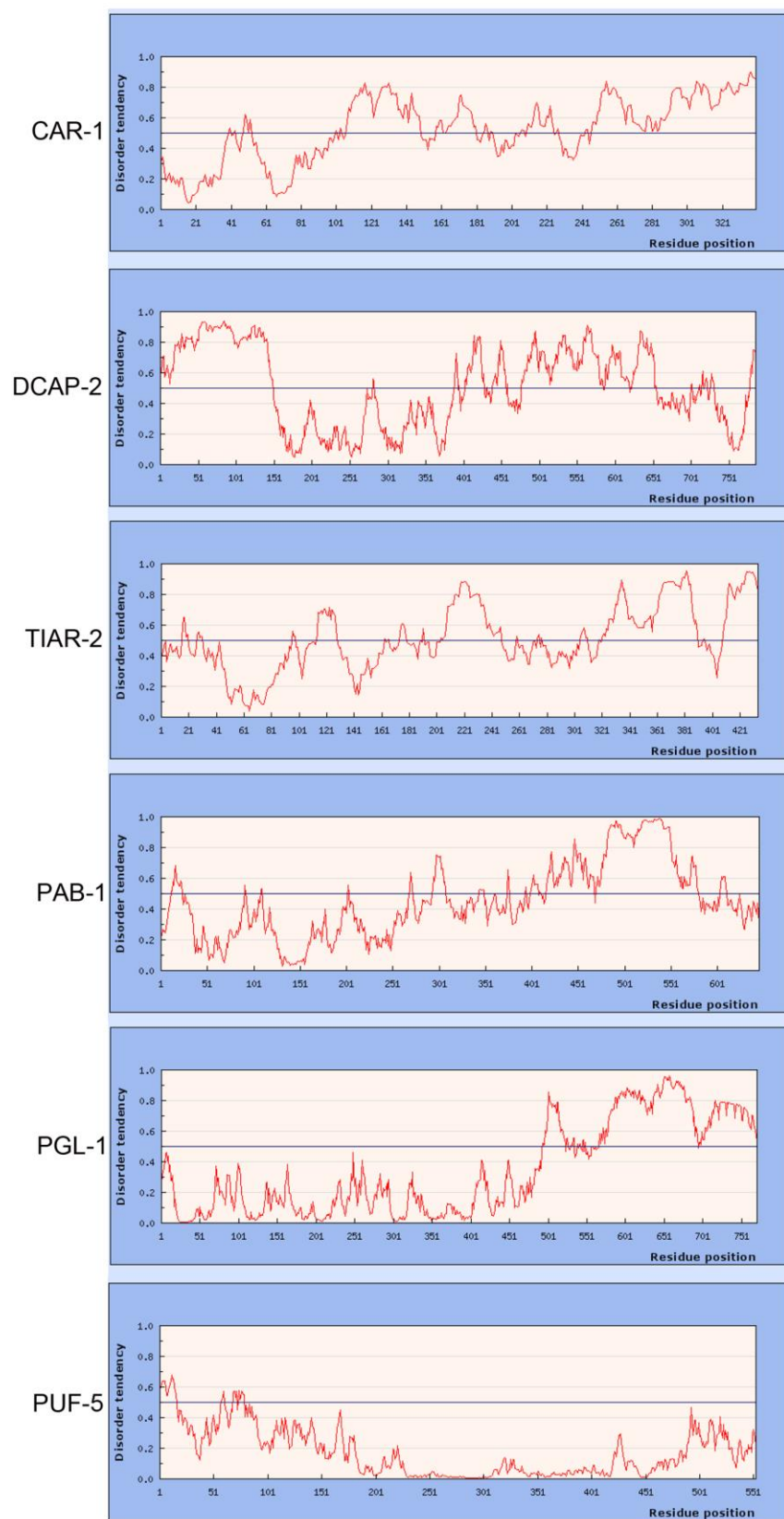
Figure S1. The majority of RNP granule protein components have IDRs. IDRs were identified using IUPRED (Dosztanyi et al. 2005). The disorder tendency was >0.5 for at least one long sequence in CAR-1, DCAP-2, TIAR-2, PAB-1, and PGL-1, but not in PUF-5.
