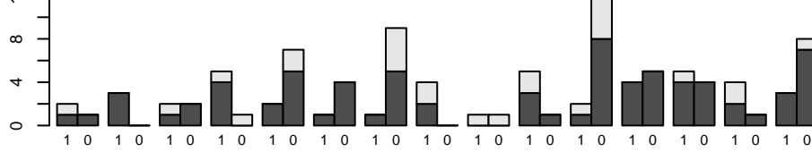
Unclassified Helcococcus
