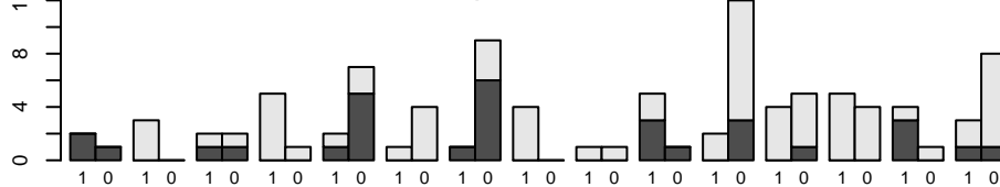
Unclassified Acinetobacter
