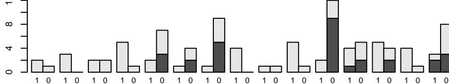
Unclassified Roseburia
