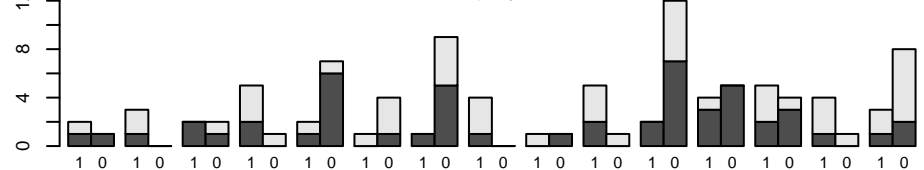
Unclassified Porphyromonadaceae
