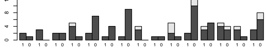
Unclassified Prevotella
