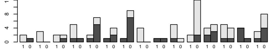
Unclassified Aerococcaceae
