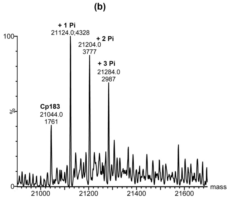
S2 Figure. ESI mass spectra phosphorylated Cp183, P-Cp183, prepared by co-expression of Cp183 and SRPK (a) in capsids incorporating E. Coli RNA and (b) in empty capsids from purified P-Cp183. The peak labels show assignment, mass, and intensity.
