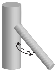
GL-bottlegrowth_div_CL-recentgrowth
