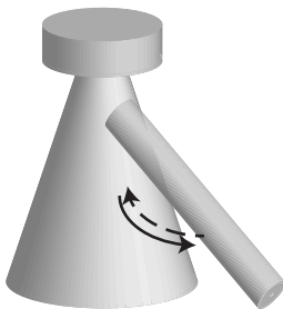
GL-bottlegrowth_div_CL-pastgrowth
