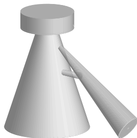
GL-bottlegrowth_div_CL-growth_admix_noinCLmig
