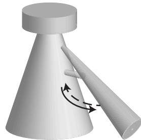
GL-bottlegrowth_div_CL-growth_admix_nomig
