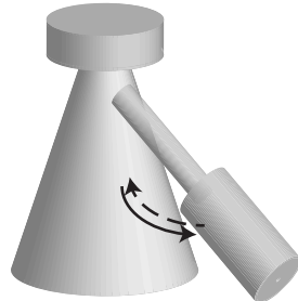
GL-bottlegrowth_div_CL-growth_admix
