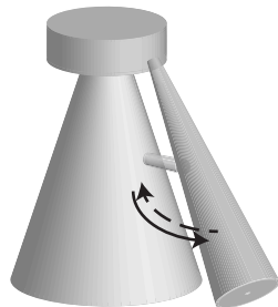
GL-bottlegrowth_div_CL-growth_admix_noinGLmig
