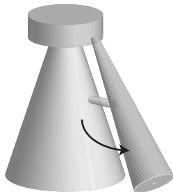
GL-bottlegrowth_div_CL-growth_admix_noinGLmig
