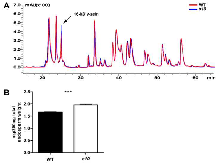
S8 Fig. HPLC analysis of the content of 16-kD \gamma -zein in the wild-type and o10 mature kernels. (A) The peak diagram of HPLC from the determination of the zein content in mature kernels of the wild-type and o10 . (B) The relative concentrations of 16-kD \gamma -zein in the wild-type and o10 mature kernels.
