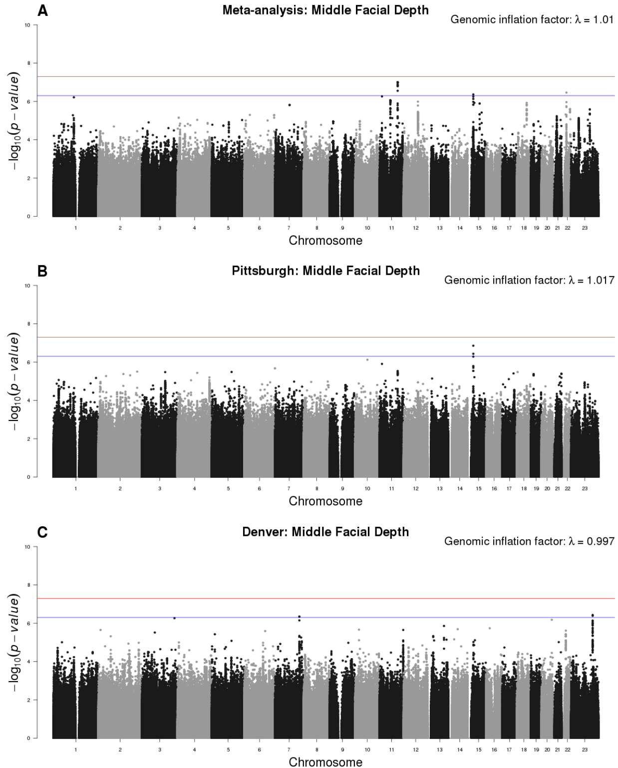
S3 Fig. Manhattan plots for middle facial depth. (A) meta-analysis results, (B) Pittsburgh sample results, and (C) Denver sample results. Lines for p-value thresholds set at 5 \times 10^{-8} for genome-wide significance and 5 \times 10^{-7} for suggestive significance
