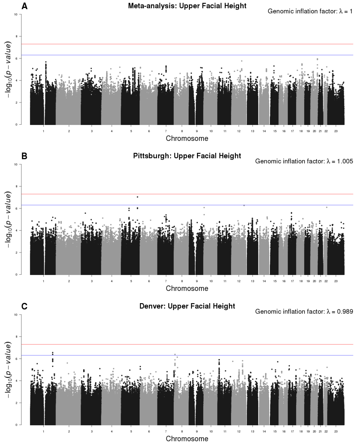
S6 Fig. Manhattan plots for upper facial height. (A) meta-analysis results, (B) Pittsburgh sample results, and (C) Denver sample results. Lines for p-value thresholds set at 5 \times 10^{-8} for genome-wide significance and 5 \times 10^{-7} for suggestive significance
