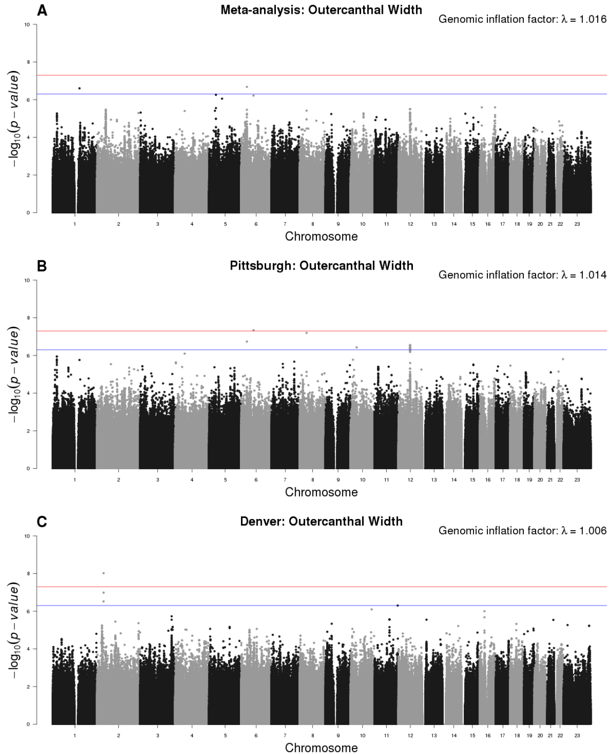
S9 Fig. Manhattan plots for outercanthal width. (A) meta-analysis results, (B) Pittsburgh sample results, and (C) Denver sample results. Lines for p-value thresholds set at 5 \times 10^{-8} for genome-wide significance and 5 \times 10^{-7} for suggestive significance.
