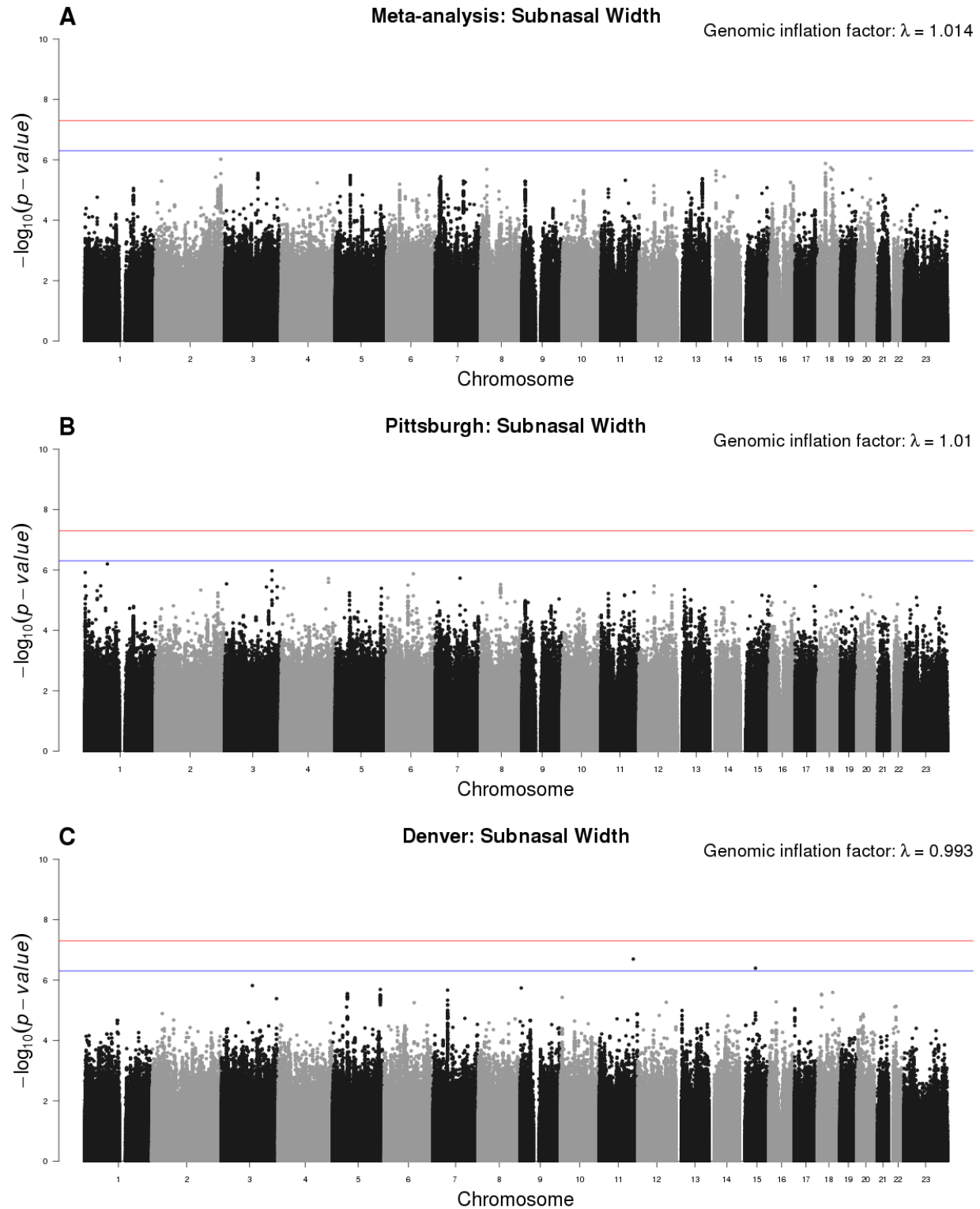
S12 Fig. Manhattan plots for subnasal width. (A) meta-analysis results, (B) Pittsburgh sample results, and (C) Denver sample results. Lines for p-value thresholds set at 5 \times 10^{-8} for genome-wide significance and 5 \times 10^{-7} for suggestive significance.
