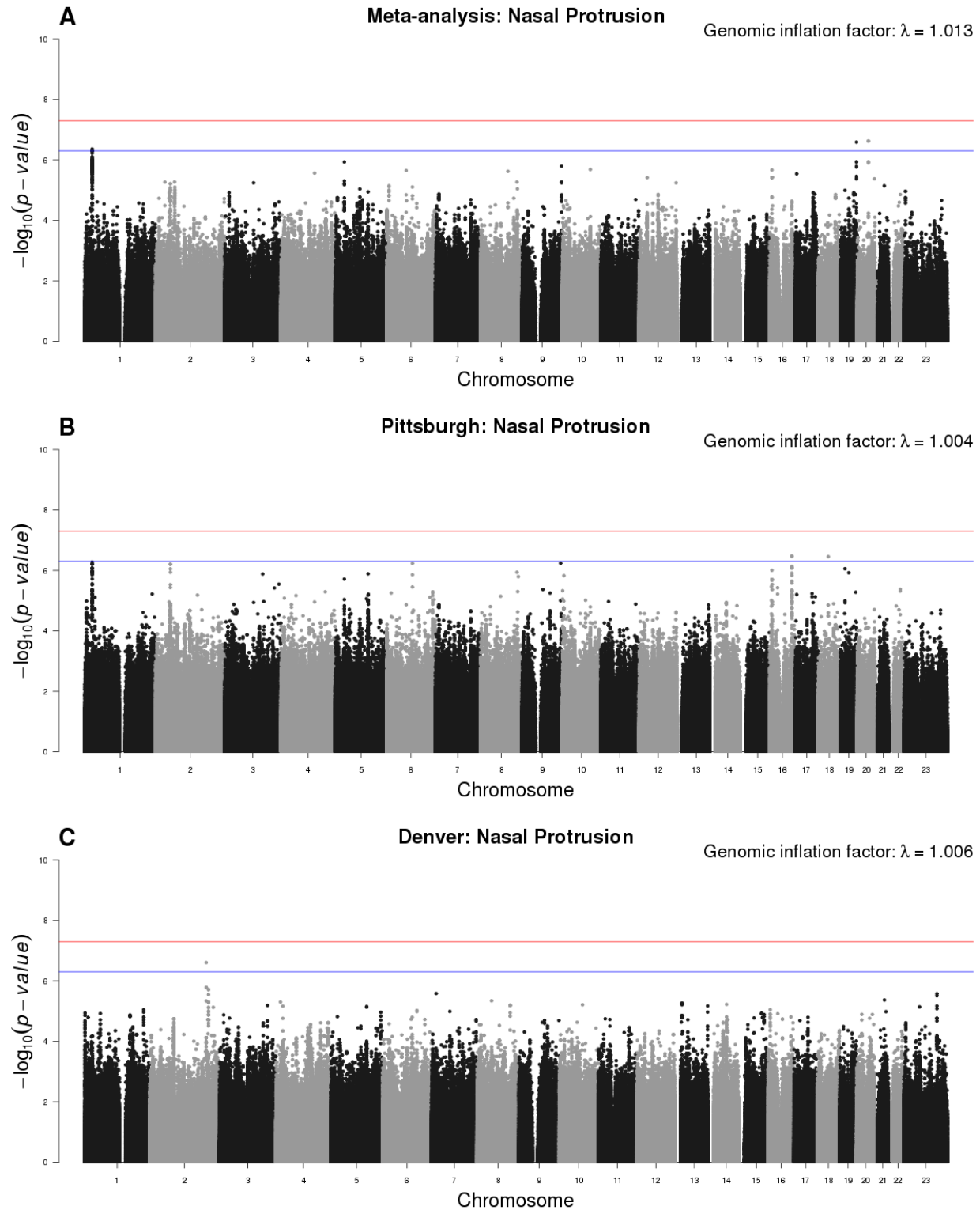
S13 Fig. Manhattan plots for nasal protrusion. (A) meta-analysis results, (B) Pittsburgh sample results, and (C) Denver sample results. Lines for p-value thresholds set at 5 \times 10^{-8} for genome-wide significance and 5 \times 10^{-7} for suggestive significance.
