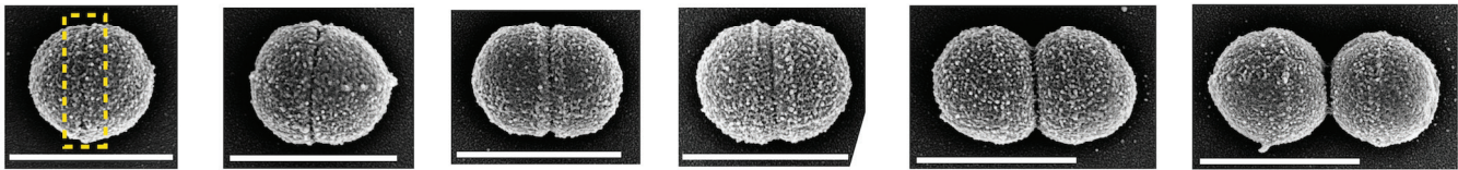
Jeotgalicoccus sp.
