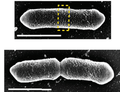
Listeria monocytogenes
