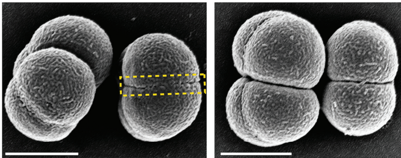
Sporosarcina ureae
