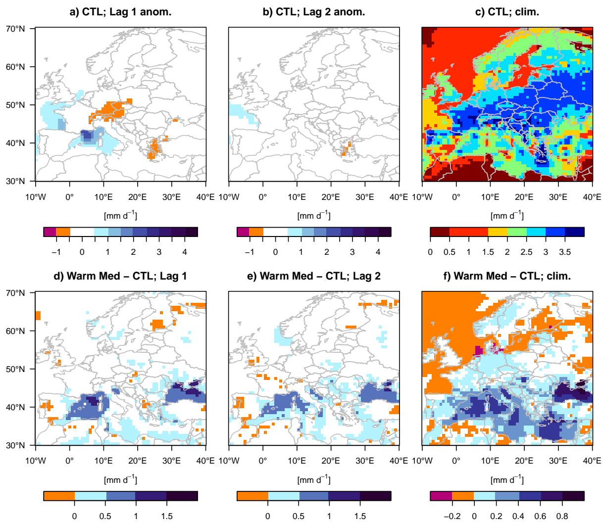
Figure S10: Evaporation . Same as Fig. S8 but for evaporation ( \text{mm d}^{-1} ). Maps created with R version 3.2.3 ( www.r-project.org ).
