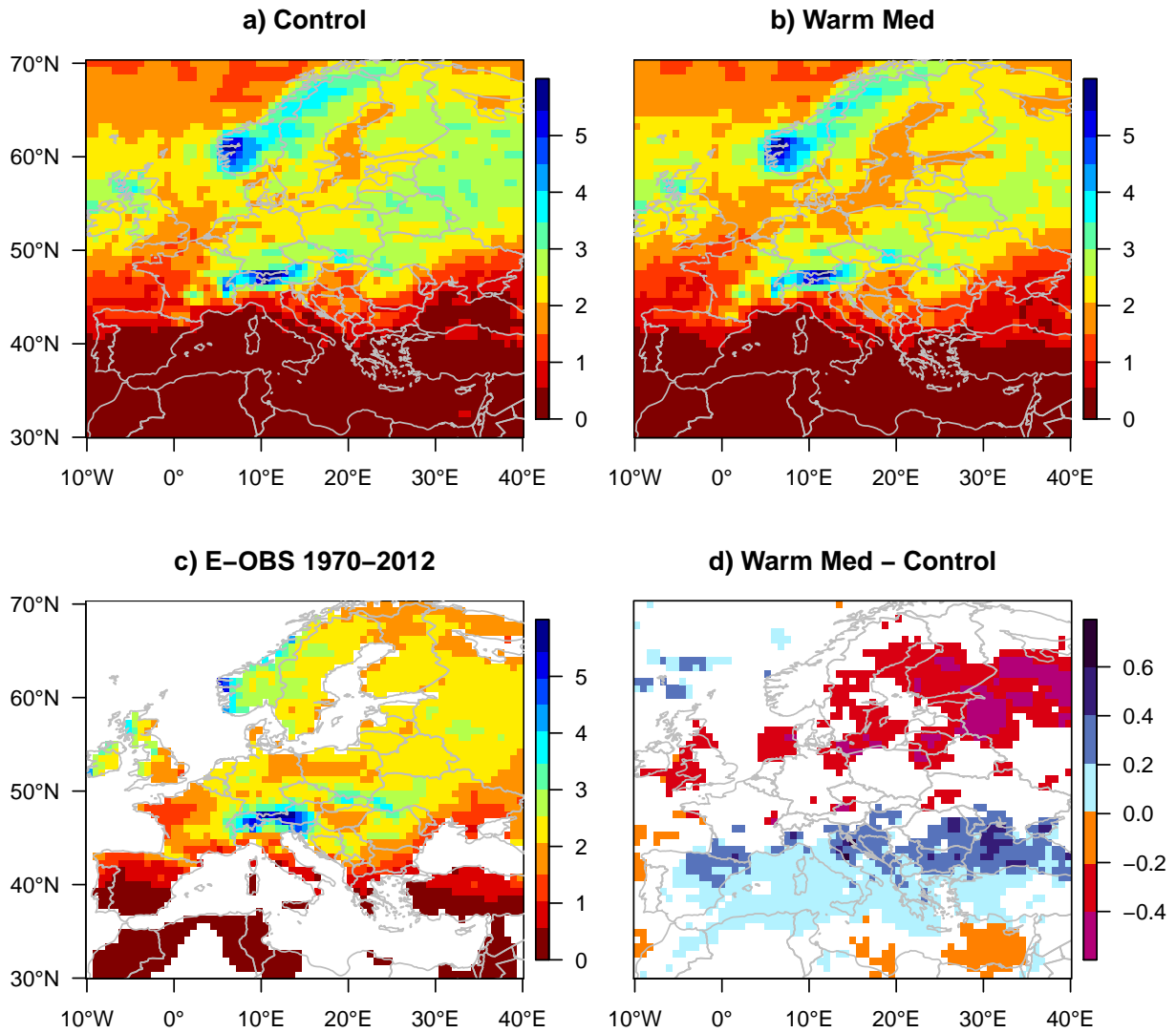
Figure S1: Summer mean precipitation. Mean JJA precipitation (mm/day) in (a) control experiment, (b) warm Mediterranean (Med warm ) experiment, and (c) E-OBS, version 10. (d) Significant differences between JJA-climatology in Med warm and control. Maps created with R version 3.2.3 ( www.r-project.org ).
