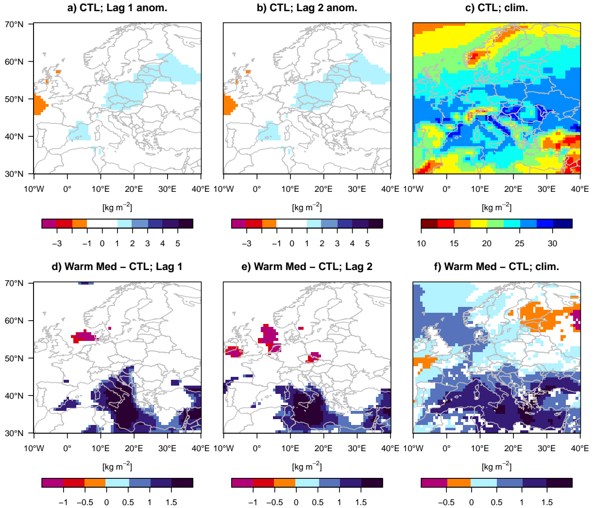
Figure S8: Precipitable water. Composites of column integrated precipitable water ( \text{kg m}^{-2} ) on (a, d) lag 1 and (b, e) lag 2 days before heavy-precipitation events: (a, b) anomalies in control experiment (relative to climatology) and (d, e) significant differences between composites in Med warm and control. (c) JJA-climatology of control experiment. (f) Significant differences between JJA-climatology in Med warm and control. Maps created with R version 3.2.3 ( www.r-project.org ).
