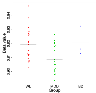
cg01642827 (GET4)
