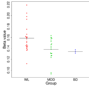
cg08608800 (ZC3H13)
