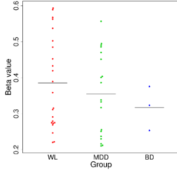
cg18995182 (COL4A5/6)
