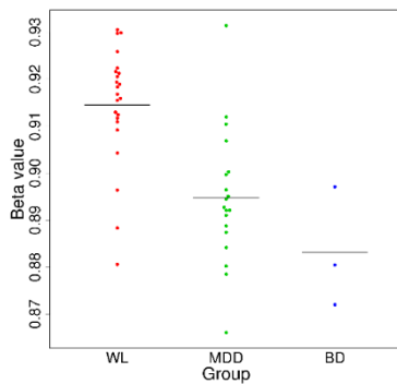
cg26893134 (FRK)
