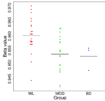
cg19199483 (N/A)
