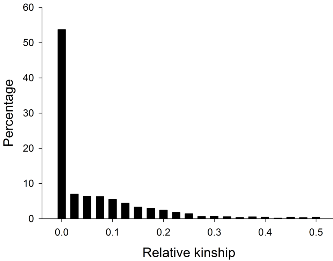
Supplemental Fig.2. Distribution of pairwise relative kinship coefficients between 72 rice varieties.
