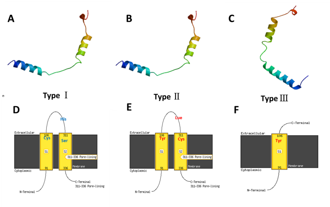
Supplemental Fig.3. Secondary and transmembrane structures of protein types I, II, and III.
