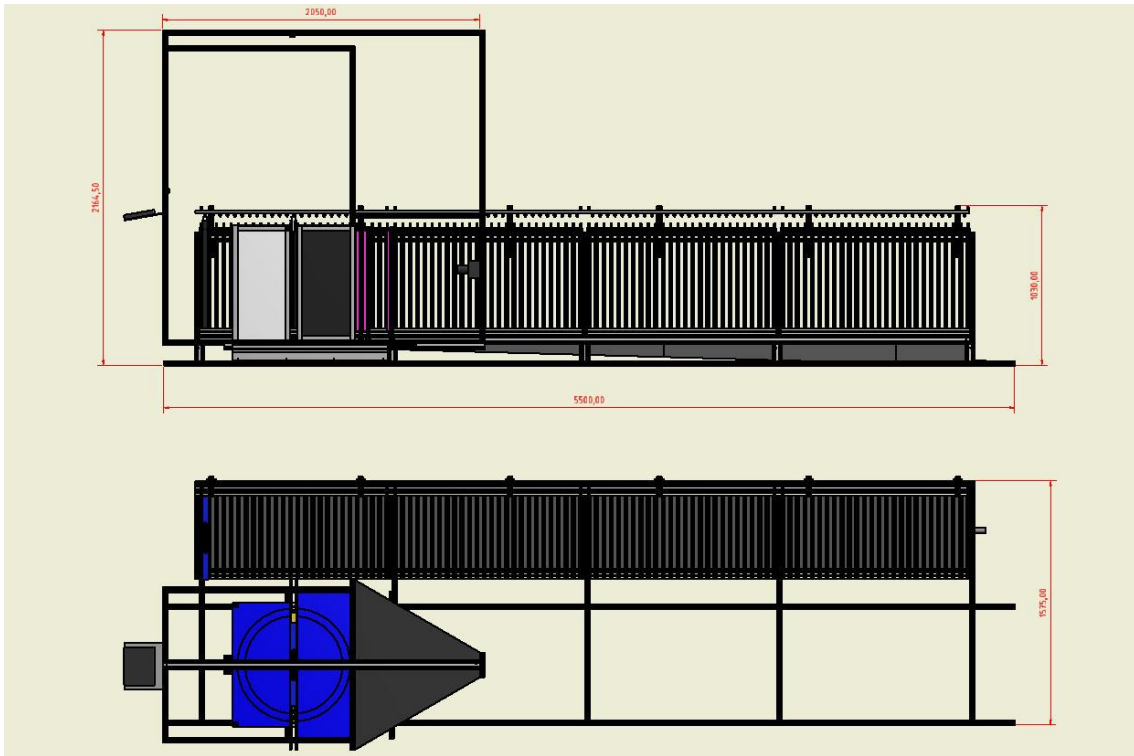
Additional file 1: Construction drawing of the RADIX platform (units:mm).
