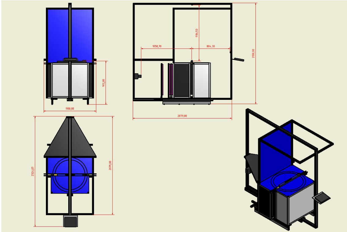
Additional file 2: Constructional drawing of the imaging station (units:mm).
