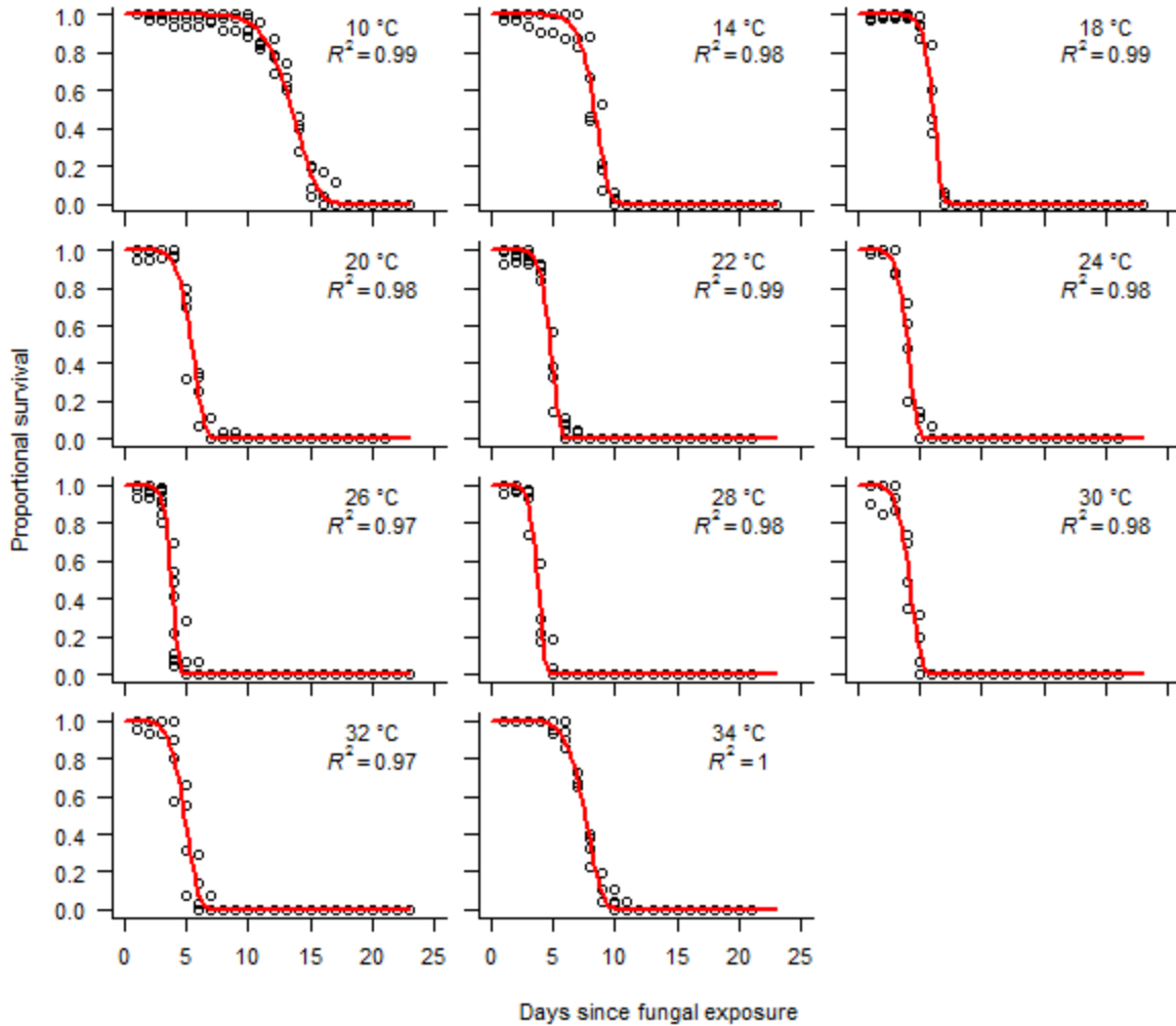
Fig. S1. Graphical evaluation of Weibull parameter fits of corrected mosquito survival at the high fungal application rate. Points represent corrected daily proportional survival from treatment replicates, and lines represent best fit curves for each temperature treatment with the associated R^2 noted in the legend. Similarly high R^2 values were obtained for the fits of the low application rate survival data ( R^2=0.95-0.99 , curves not shown).
