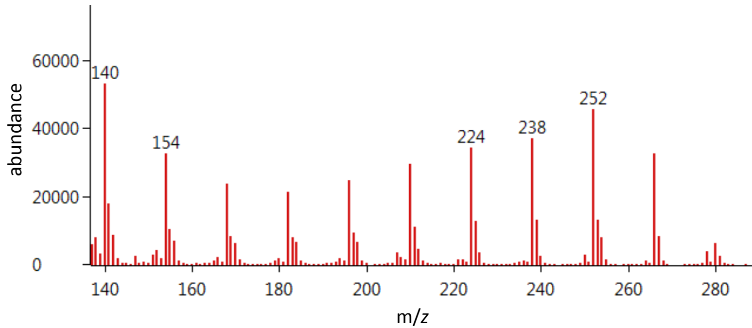
S1 Fig. MS spectrum from the peak labeled lipid in the GC/MS shown in Fig 2 panel B. This characteristic fragmentation pattern of 14 Da. increments is highly indicative of a long chain fatty acid.
