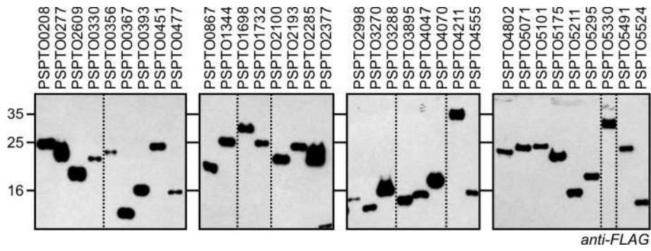
Figure S2. Anti-FLAG western blot of purified small secreted non-annotated proteins. Small secreted non-annotated proteins were expressed from pTSGAT1 in E. coli as FLAG-His-tagged proteins and purified on Ni-NTA columns. Proteins were separated on protein gels, transferred onto a PVDF membrane and detected with anti-FLAG antibodies.
