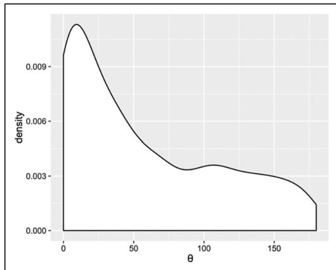
Supplementary Fig. S1. Density of theta differences between pairs of cell lines. A density plot of theta values from Figure 4 , indicating most cell lines responded very similar to one another when treated with the same compounds, demonstrated by the abundance of low theta values.
