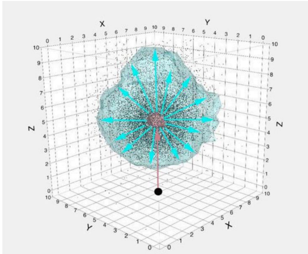
Supplementary figure 1. Three-dimensional scatterplot illustrating the difference between the systemic errors of representative points of interest distribution from a starting point (black circle) presented as a red cloud and the random errors represented as a light blue cloud. The appropriate CTV-PTV and OAR-PRV margins accounts for both the systematic and random error component.
