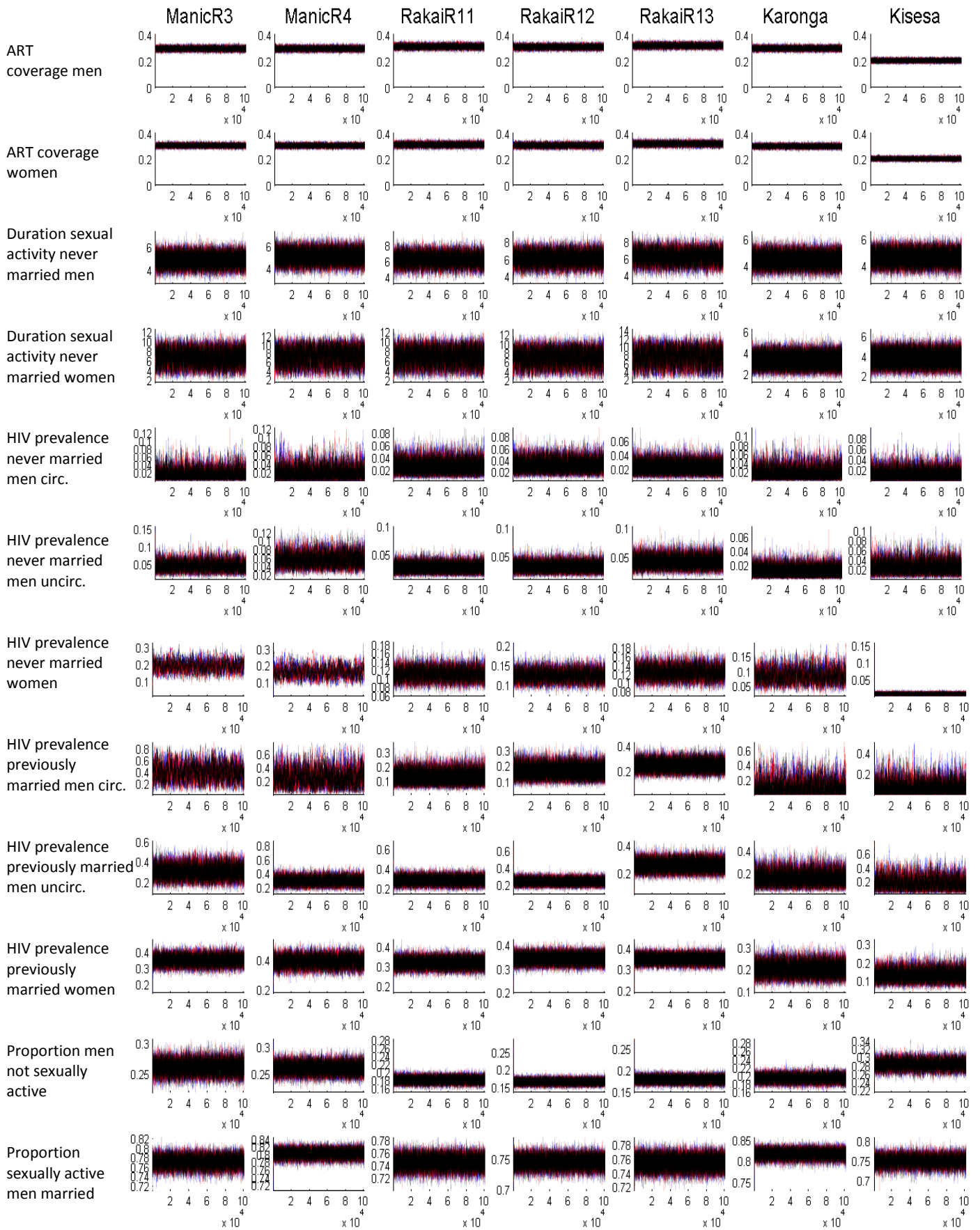
S3 Fig. Trace plots for parameters determining the ART coverage, duration of sexual activity, distribution and prevalence per group.
