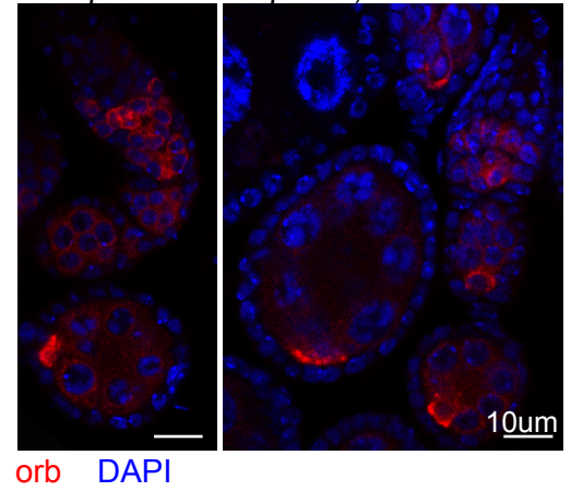
I oocyte axis patterning
