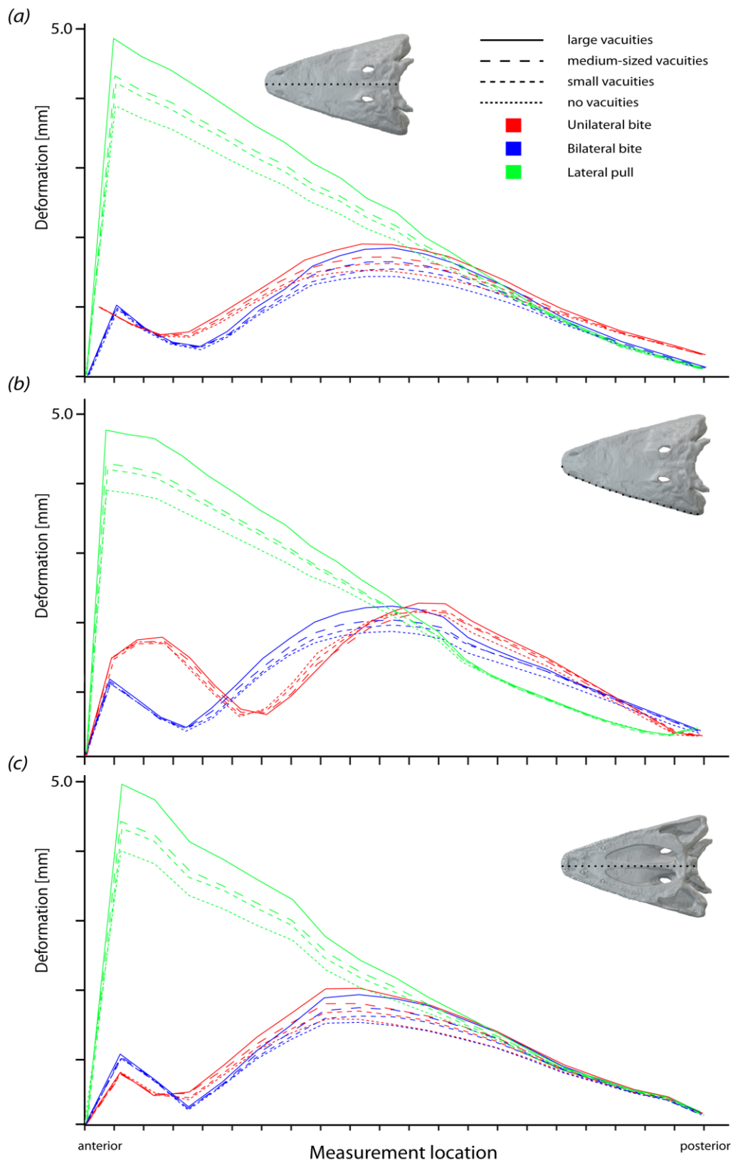
Supplementary figure 7 Deformation magnitudes for different tested cranial configurations. Measured along (a) the skull roof, (b) the left lateral margin, (c) the ventral midline.
