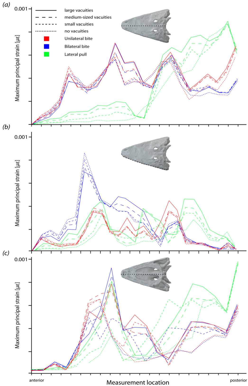
Supplementary figure 8 Maximum principal strain magnitudes for different tested cranial configurations. Measured along (a) the skull roof, (b) the left lateral margin, (c) the ventral midline.
