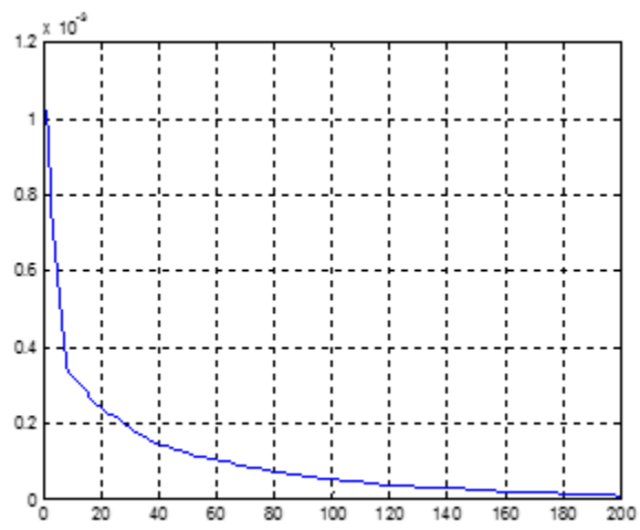
Eigenvalues of the Correlation Matrix of Topic Scores
