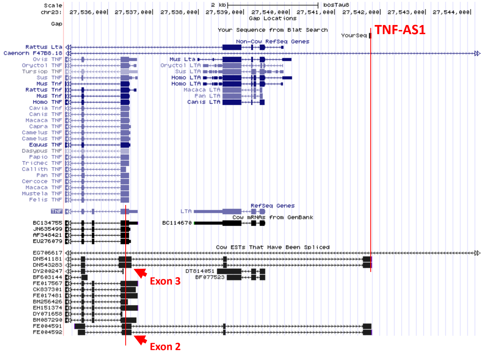
Fig. S2: UCSC Genome Browser output for bosTau8, chromosome 23, position 27,535,000-27,544,000.
