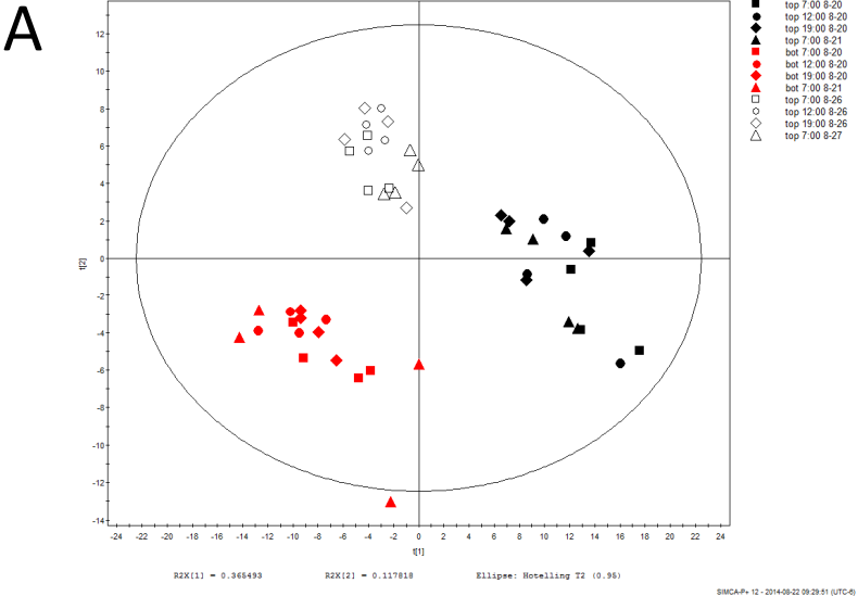
Autoscale and log transformation for A) and B) row normalization for C).
