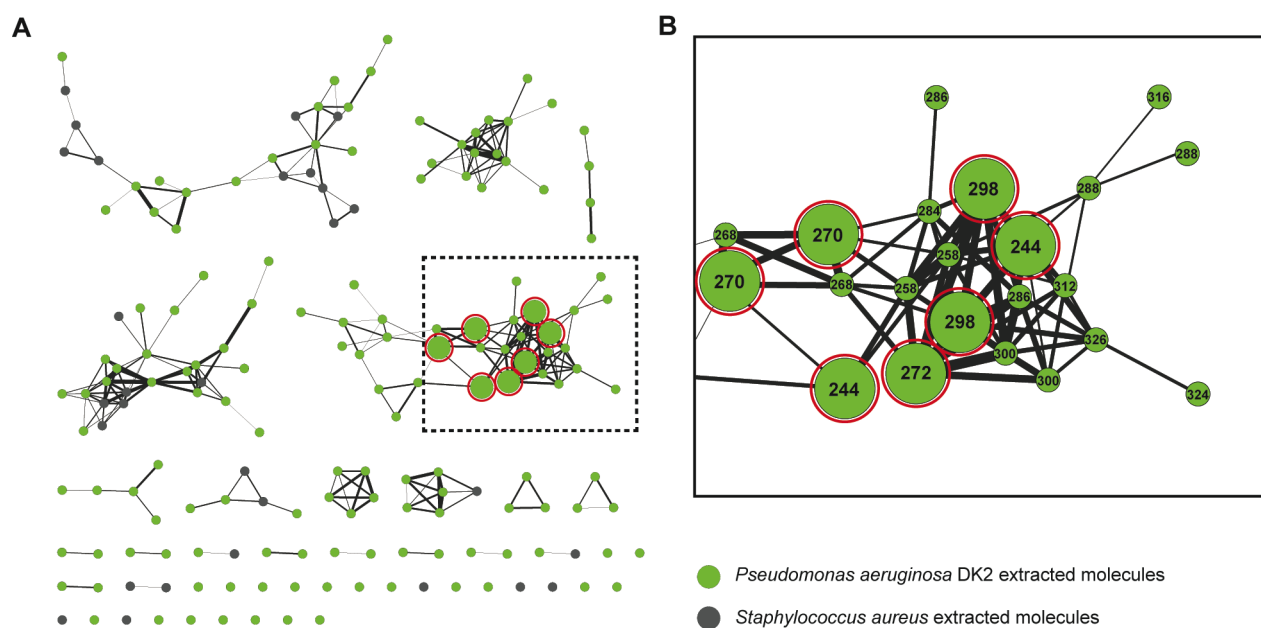
Figure S2. (A) A Cytoscape visualization of the molecular network based on MS/MS data obtained from P. aeruginosa DK2-P2M24-2003- S. aureus interaction after 48 hours co-culturing. Green nodes represent the parent masses for P. aeruginosa DK2-P2M24-2003 ( DK2 ) extracted molecules and dark grey nodes represent parent masses for S. aureus extracted molecules. The thickness of the edges between connecting nodes indicates the level of similarity. (B) Annotated molecular network of HAQ molecules extracted from P. aeruginosa DK2-P2M24-2003. Nomenclature and parent masses for the enlarged green nodes with red border are represented in Fig. 4 in the main manuscript.
