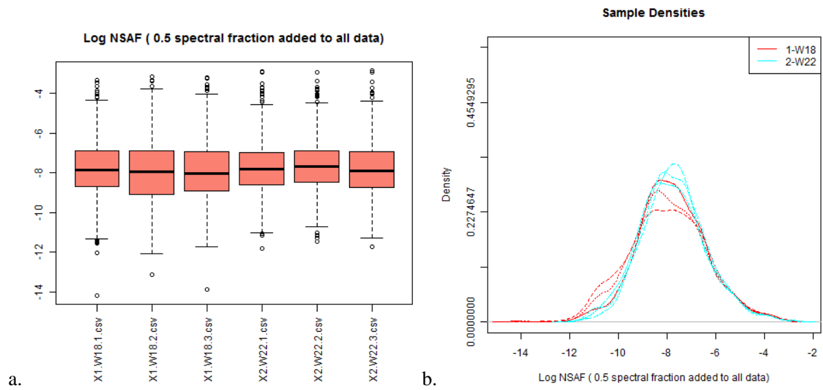
Supplementary figure S1: Distribution of log transformed NSAF values of strain WH8102 at 18°C and 22°C. a. boxplot depicting population means of replicates within and between 18°C and 22°C; b. kernel density plots depicting the normal distribution of replicate datasets.
