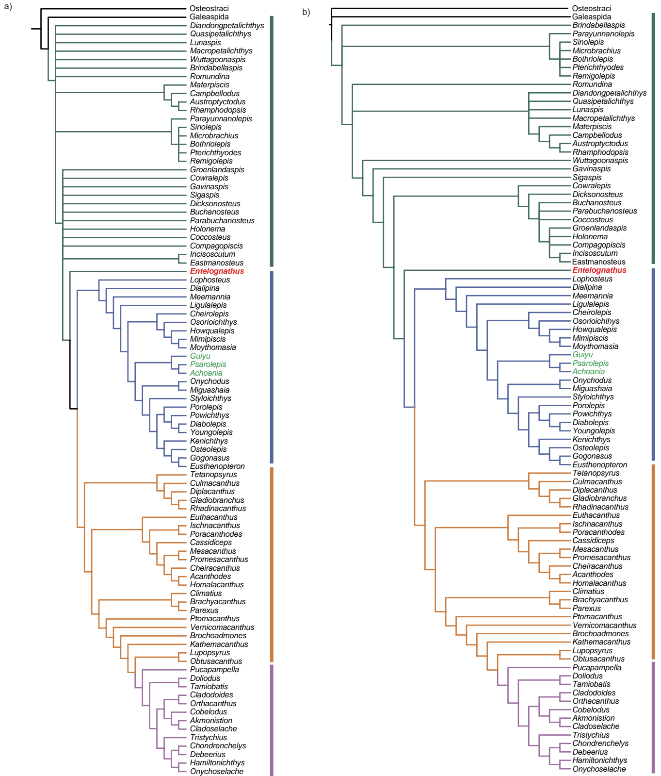
Figure S5. The strict consensus tree (a) and the 50% majority consensus tree (b) of 532 most parsimonious trees based on the dataset revised from Long et al. (2015) (total 91 taxa).
