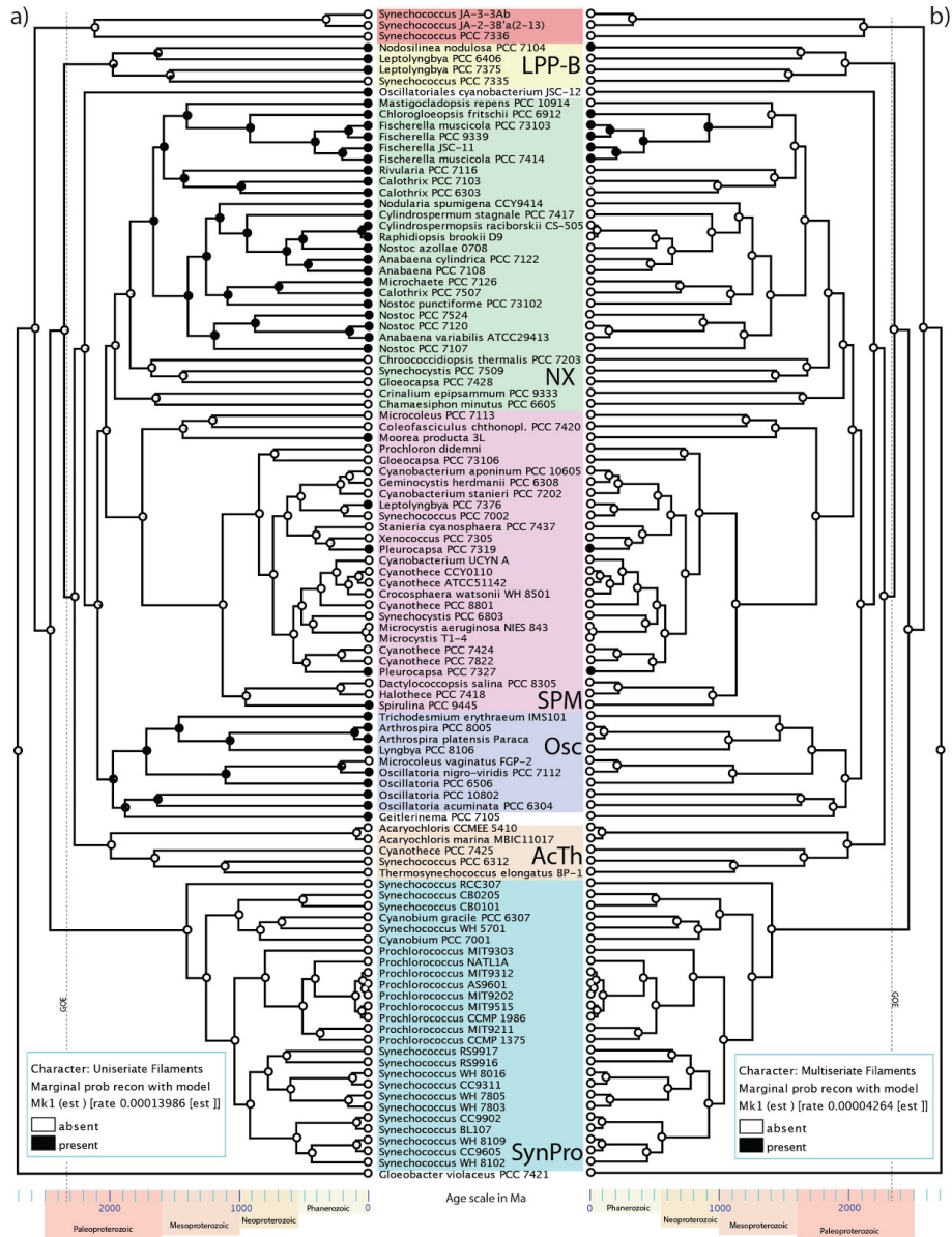
S9 Fig. Ancestral state reconstruction of uniseriate and multiseriate trichomes.
