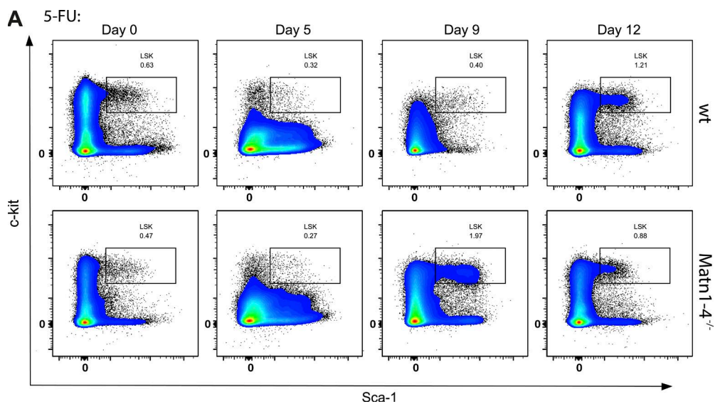
Figure S1. Gating scheme used to gate on LSK cells after 0, 5, 9, and 12 d of 5-FU treatment.
