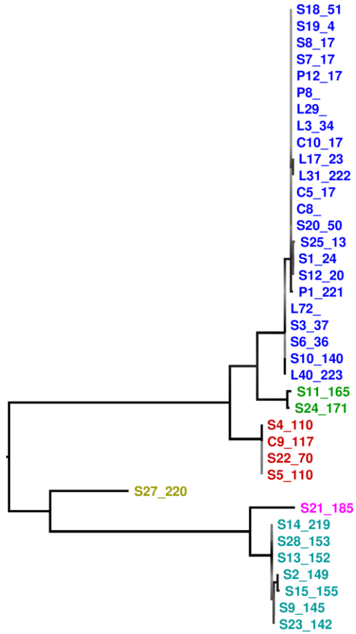
D - tpiA
