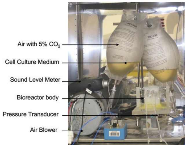
SUPPLEMENTARY FIG. S1. Picture of the bioreactor system during phonation. The bioreactor system consists of the bioreactor body mounted on a Plexiglas base connected to an air blower, a pressure transducer, and a sound level meter, which are housed in a tissue culture incubator. The commercial incubator was used to maintain a temperature of 37°C and a relative humidity of around 95%.
