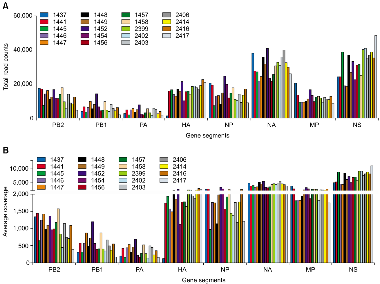
Supplementary Fig. 1. High-throughput sequencing analysis using an Ion Torrent Personal Genome Machine platform. (A) Total reads mapped in the reference genome (H5N8). (B) Average depth of coverage.
