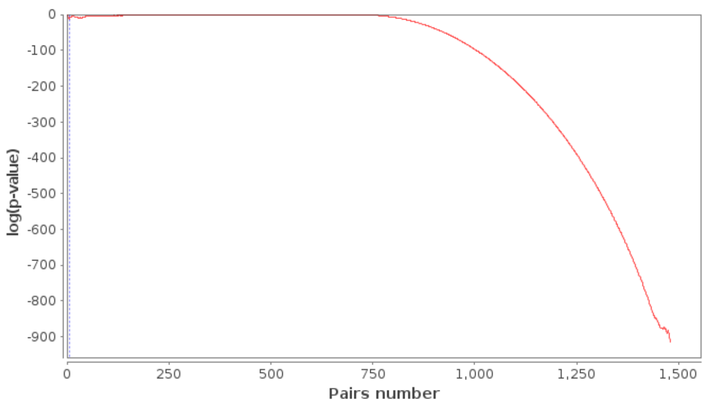
Supporting Figure S7. B-cutoff plot for shuffled regulator-site pairs
